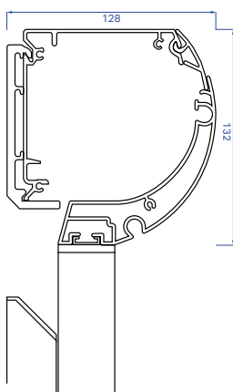
B2100 With adapter
