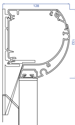
B2100 With Long end fixing bracket
