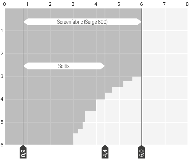
B1350 C ZIP Screen: max dimensions and application limits
