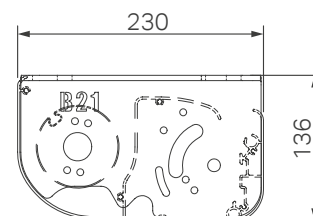
ceiling fixation B20 & B21
