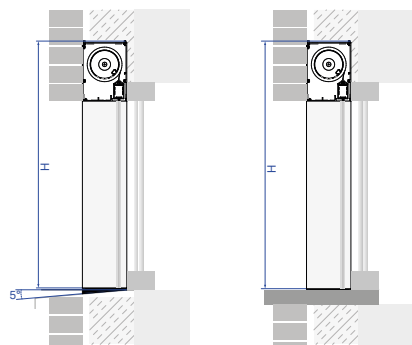
fig 1 side rail with flat end piece 5°
