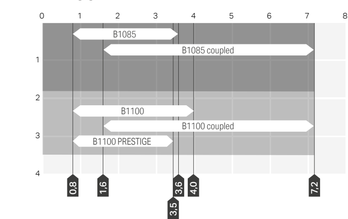
B1085 ZIP, B1100 ZIP & B1100 ZIP Prestige Screen: max dimensions and application limits
