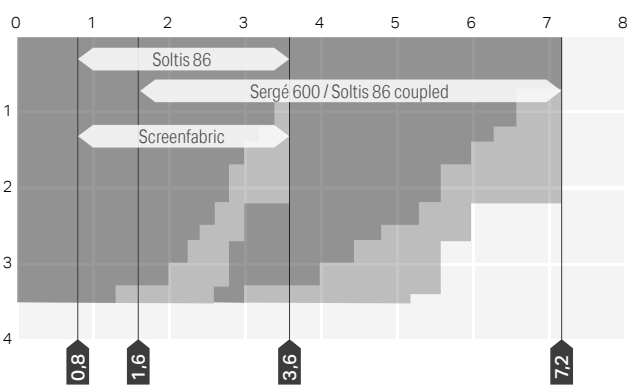
Width Height B1085 Standard screens: max dimensions and application limits
