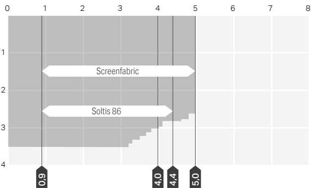
B1200 ZIP Screen: max dimensions and application limits
