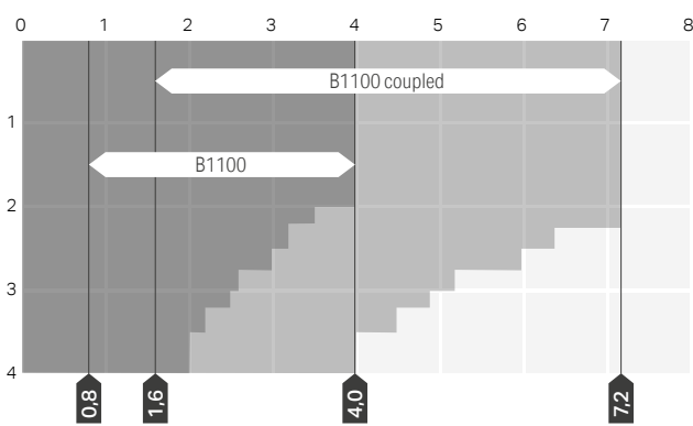
B1100 Standard screens: max dimensions and application limits
